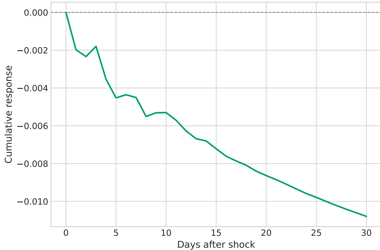
Cumulative IRF
