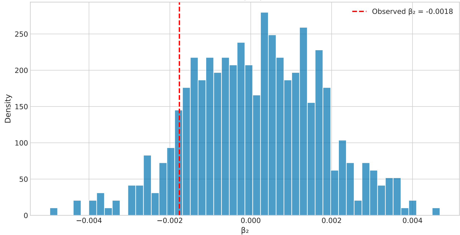
Placebo Test: \beta_2 ( p=0.2540 )
