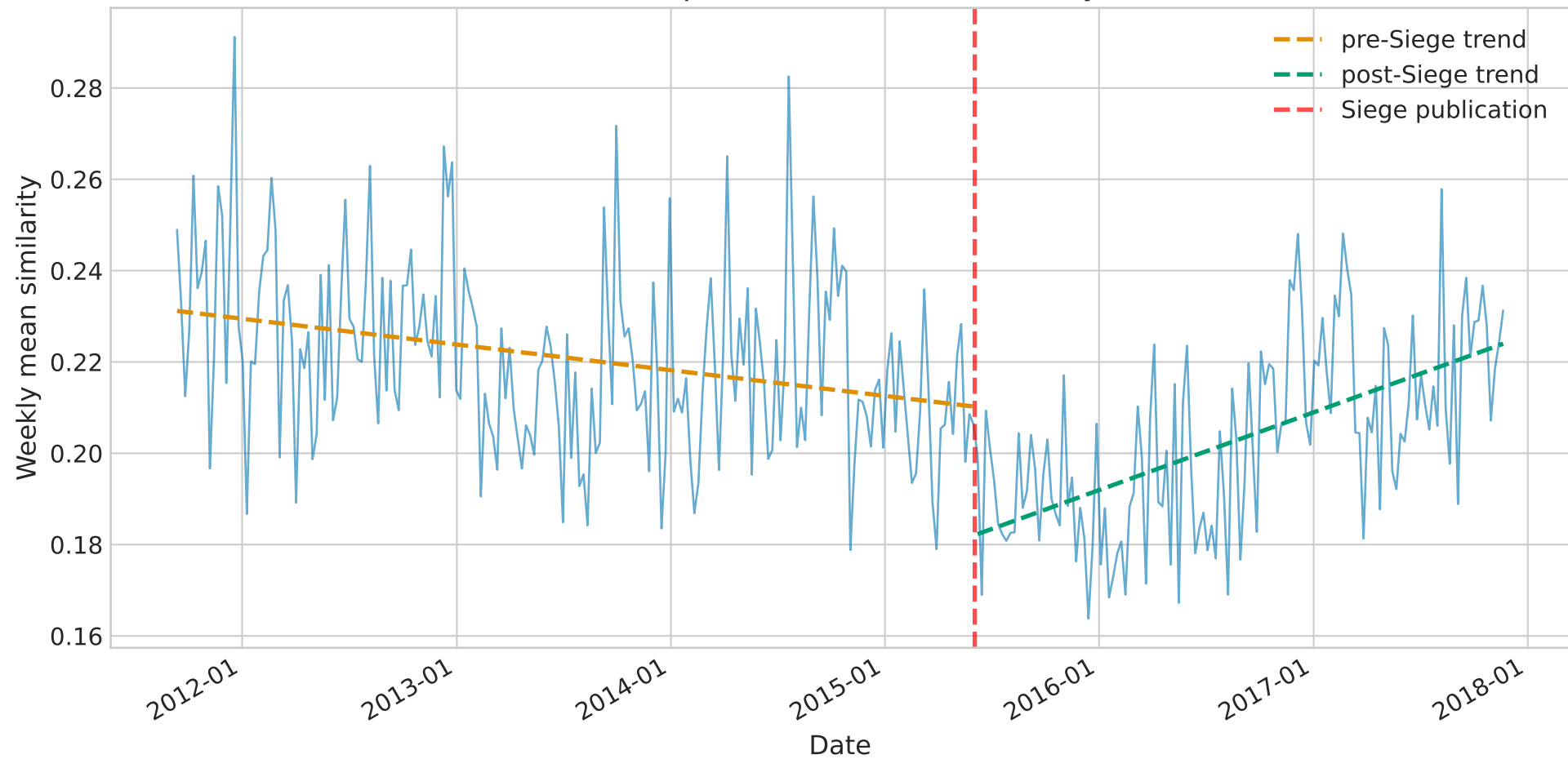
Interrupted Time Series: similarity
