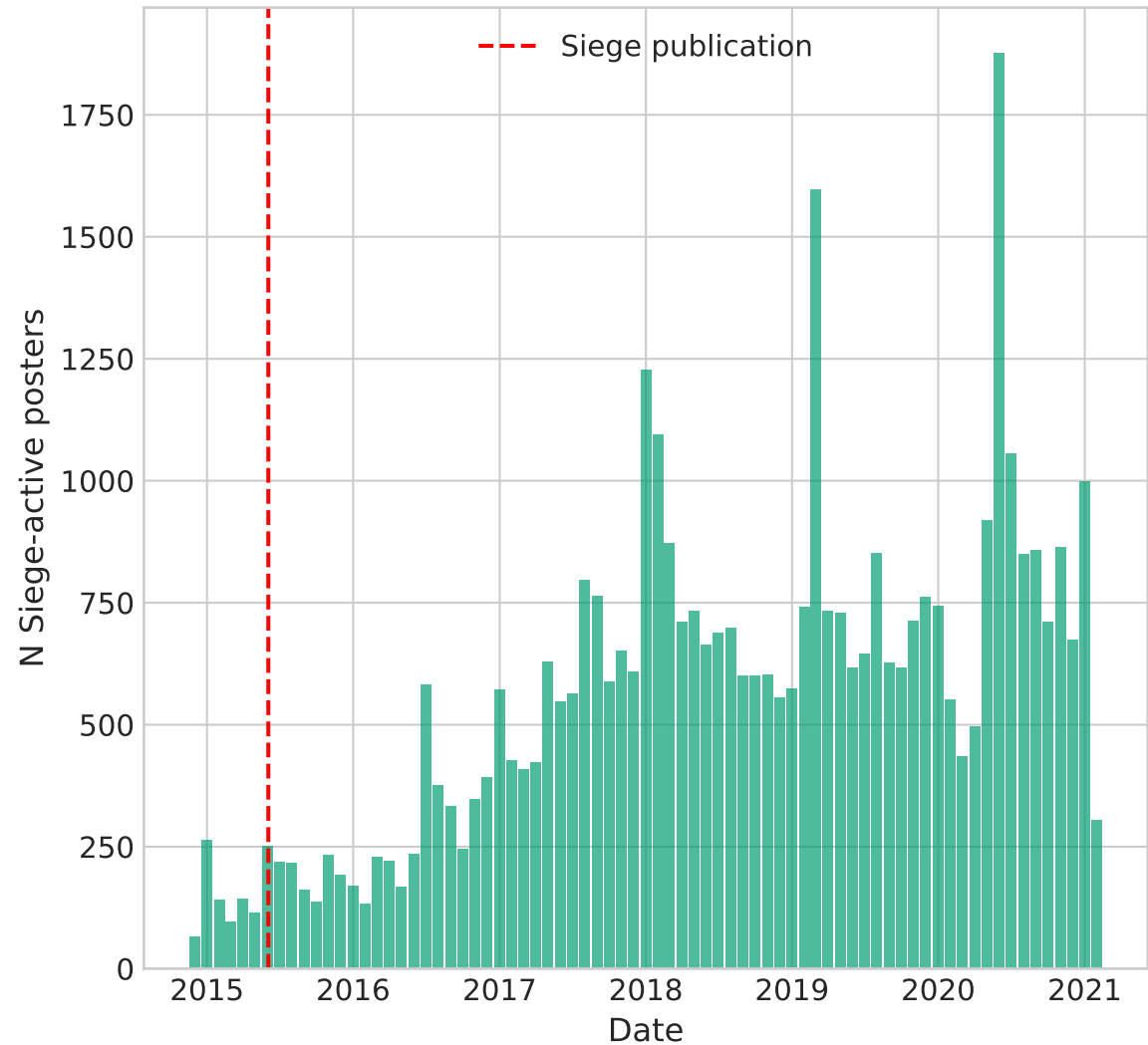
/pol/ Siege-Active Posters per Month
