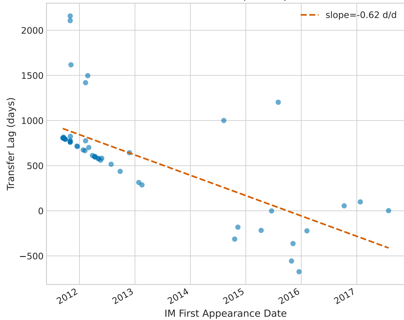
Does Transfer Speed Up?
