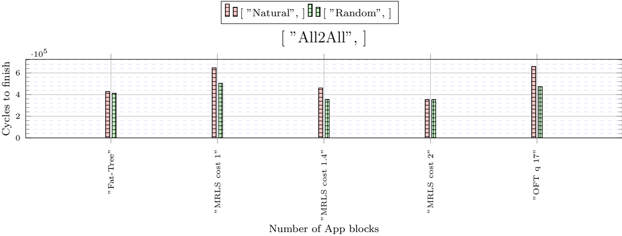
Figure 1: X: [ "All2All", ]
