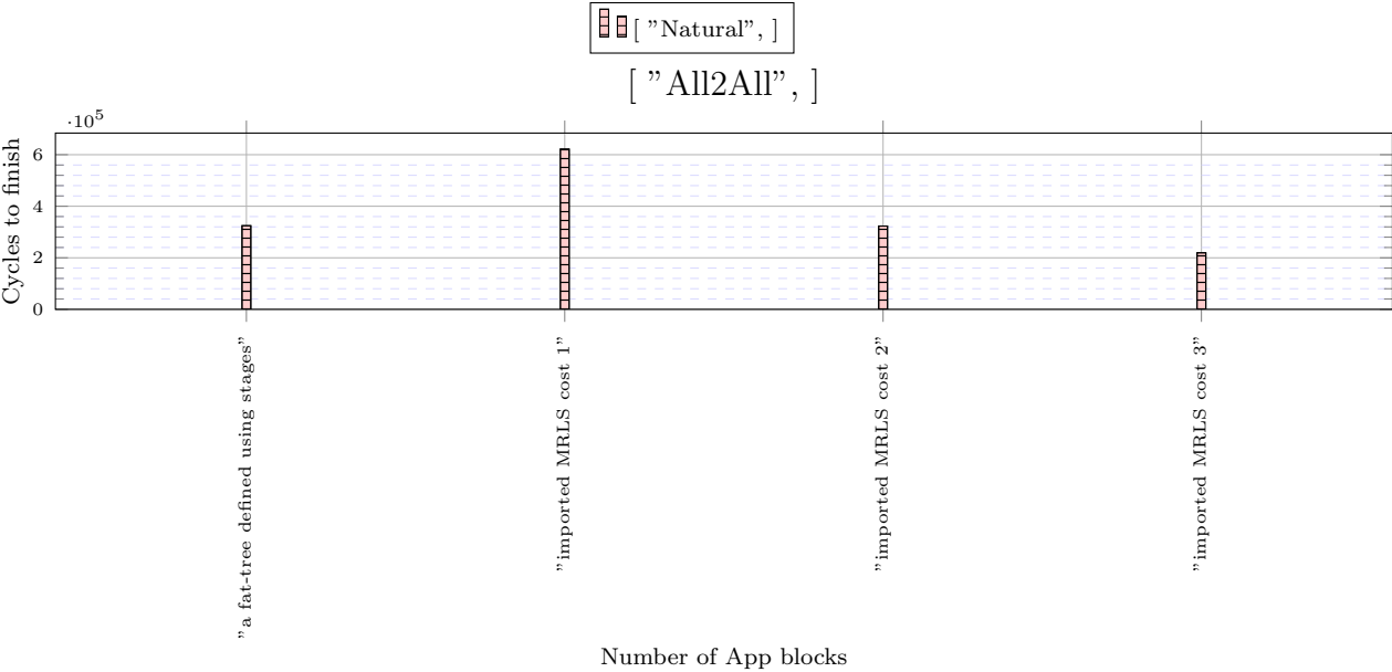
Figure 1: X: [ "All2All", ]
