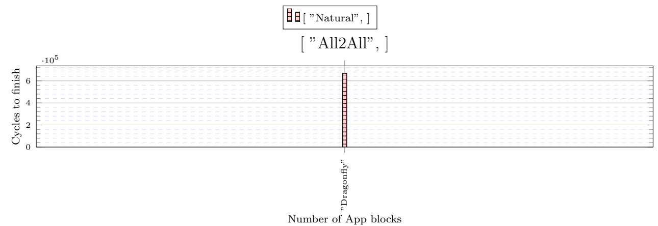
Figure 2: X: [ "All2All", ]
