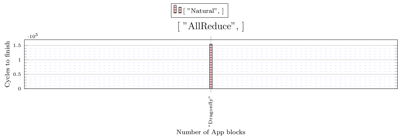
Figure 1: X: [ "AllReduce", ]
