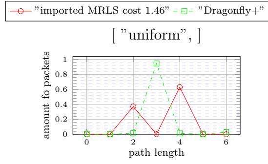
Figure 1: X: [ "uniform", ]
