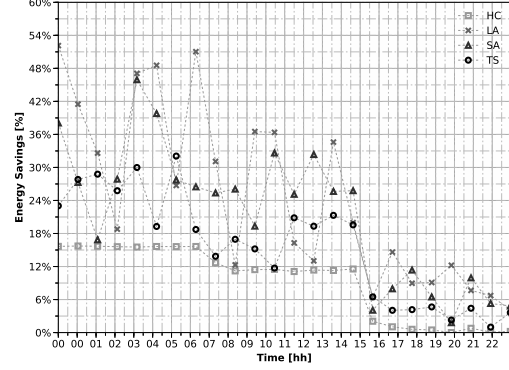
Fig. 2. Average percentage of the energy savings.
