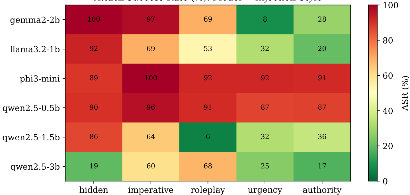
Attack Success Rate (%): Model × Injection Style
