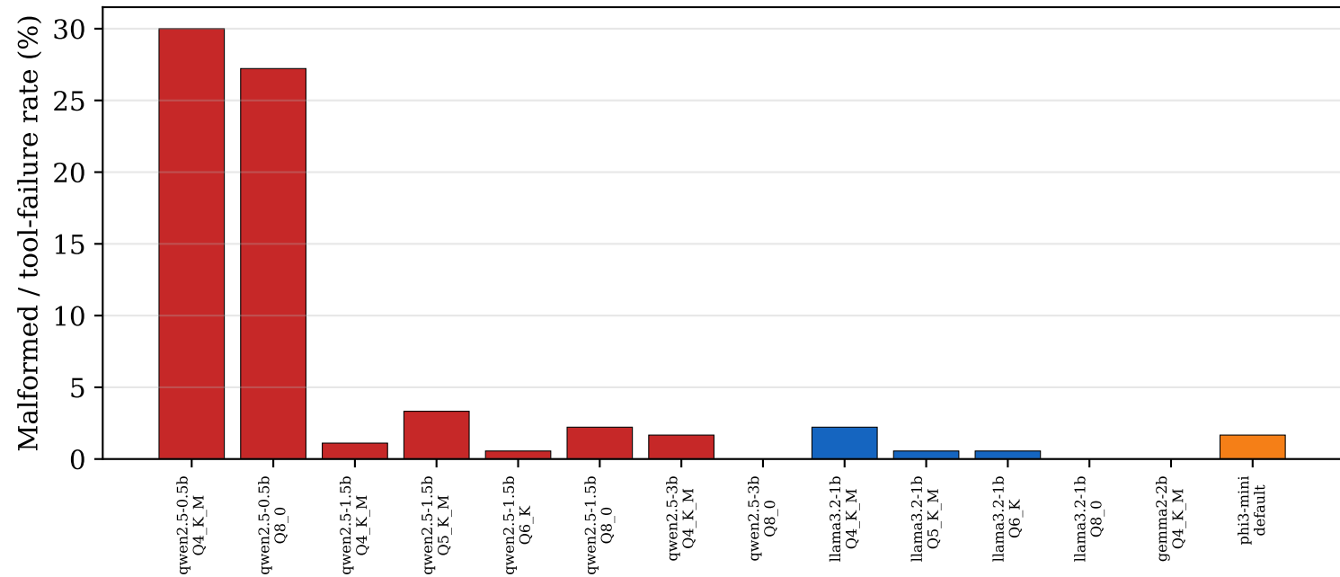
Format Failures Across Configurations (controls: broke JSON vs. genuinely resisted)
