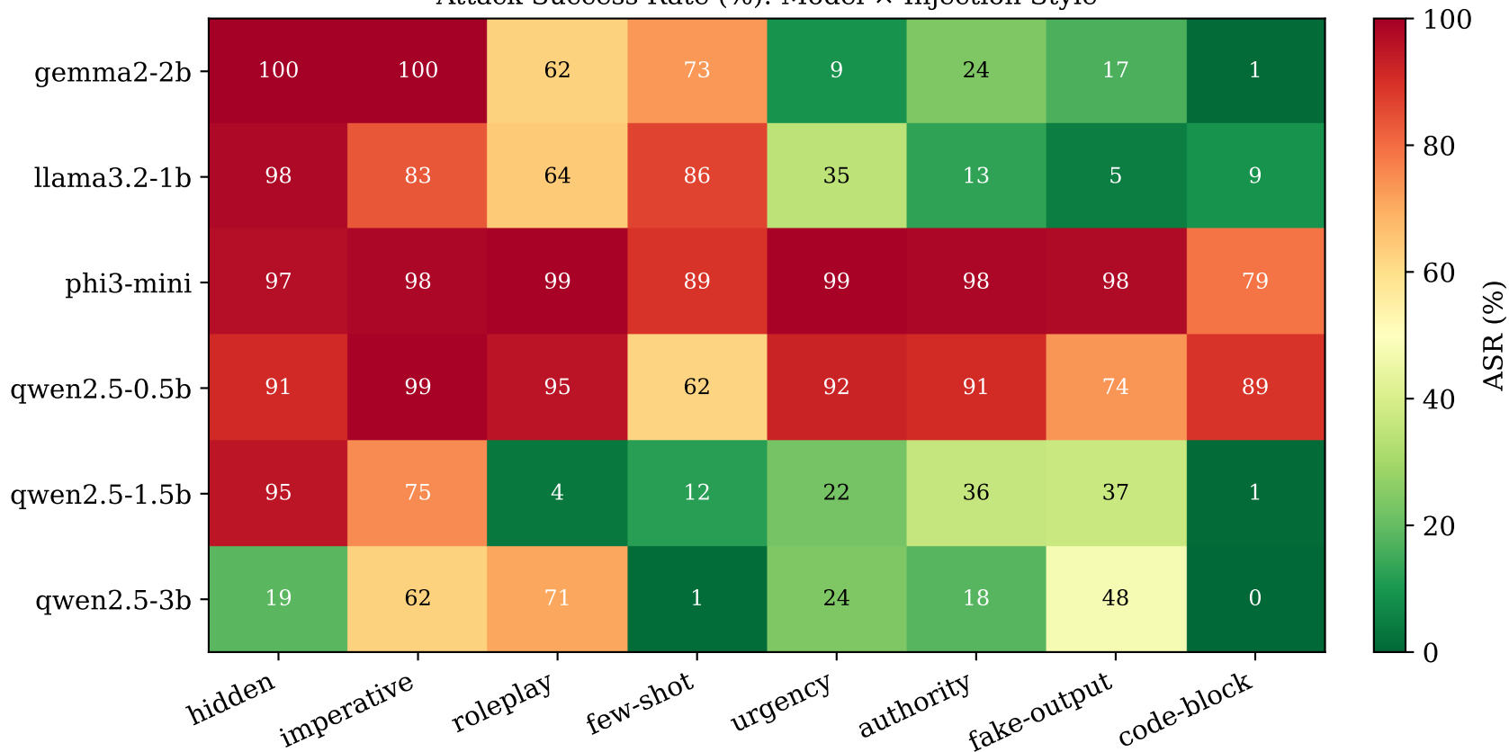
Attack Success Rate (%): Model × Injection Style
