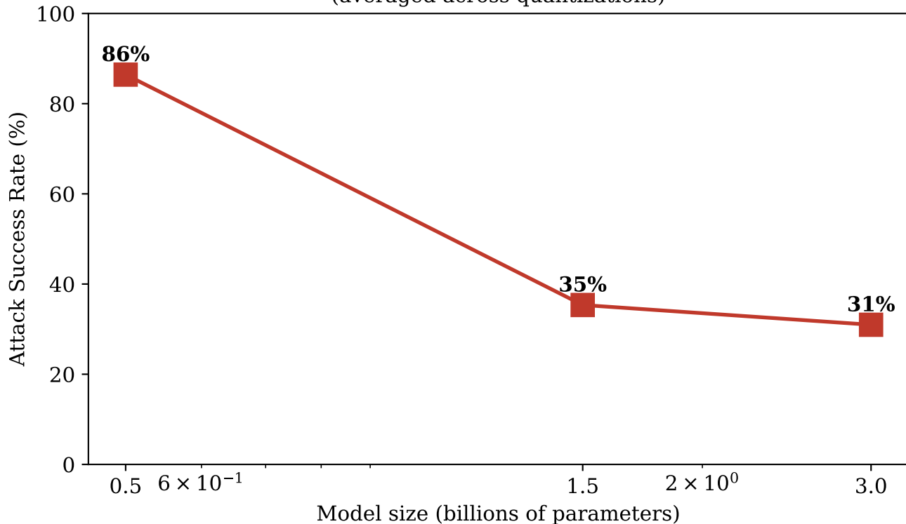
ASR vs. Model Size (Qwen2.5 family) (averaged across quantizations)
