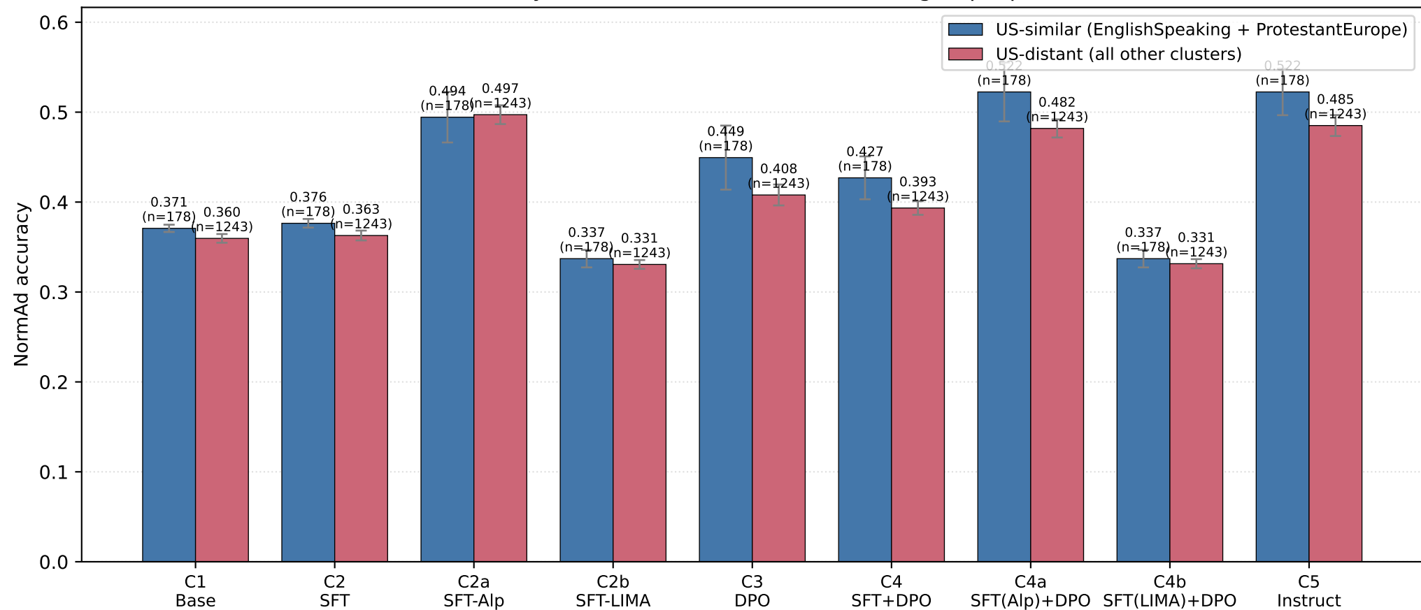
NormAd accuracy: US-similar vs US-distant cluster groups, per condition
