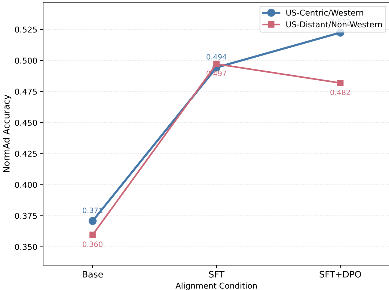
NormAd Accuracy Across Alignment Pipeline: Western vs Non-Western
