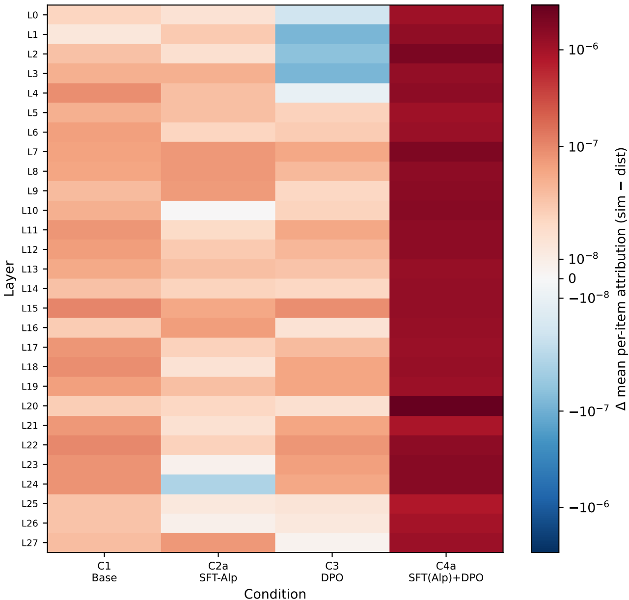
Attribution asymmetry: US-similar – US-distant (normad raw) scale: symlog (linthresh=5.50e-08)
