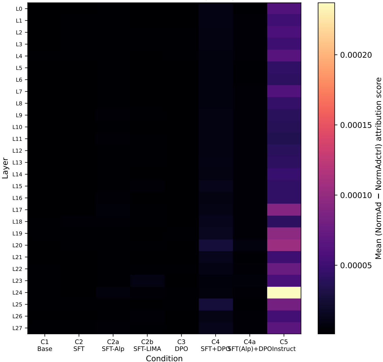
Mean culture-neuron attribution score per layer × condition
