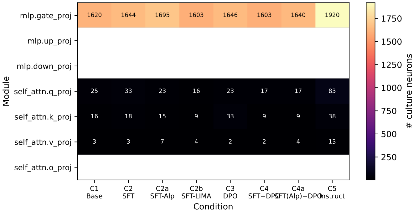
Culture-neuron count per module × condition
