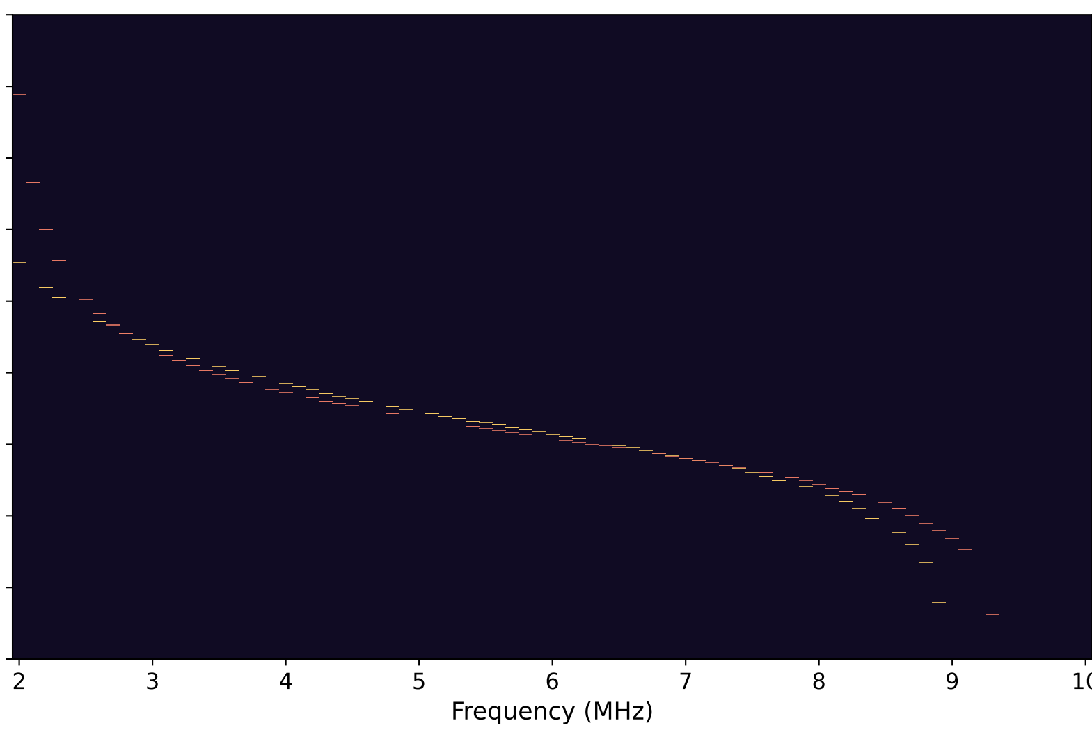
D Guarded half outer fan, 4 extra seeds · 220 returns · 57.4 s 105 anchor / 162 full directions · 220/220 reference returns matched
