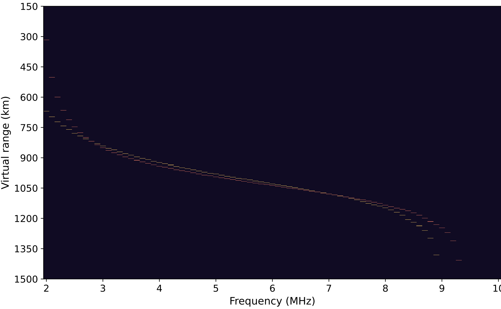
C Guarded half outer fan, 0 extra seeds · 219 returns · 41.7 s 105 anchor / 162 full directions · 219/220 reference returns matched
