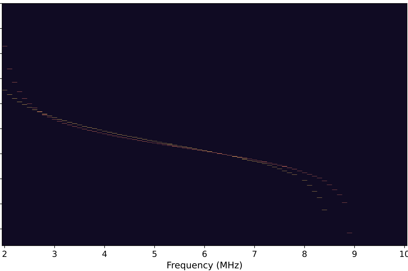
D Guarded half outer fan, 4 extra seeds · 216 returns · 70.2 s 105 anchor / 162 full directions · 215/215 reference returns matched
