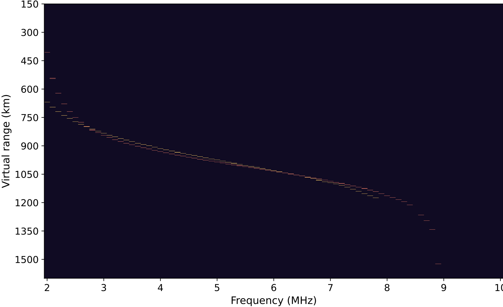
C Guarded half outer fan, 0 extra seeds · 211 returns · 45.1 s 105 anchor / 162 full directions · 208/215 reference returns matched
