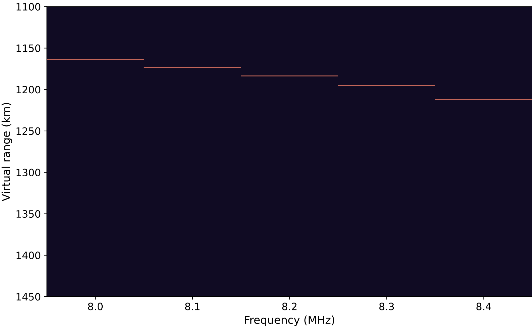
C Guarded half outer fan, 0 extra seeds · 5 returns · 45.1 s 105 anchor / 162 full directions · 5/10 reference returns matched
