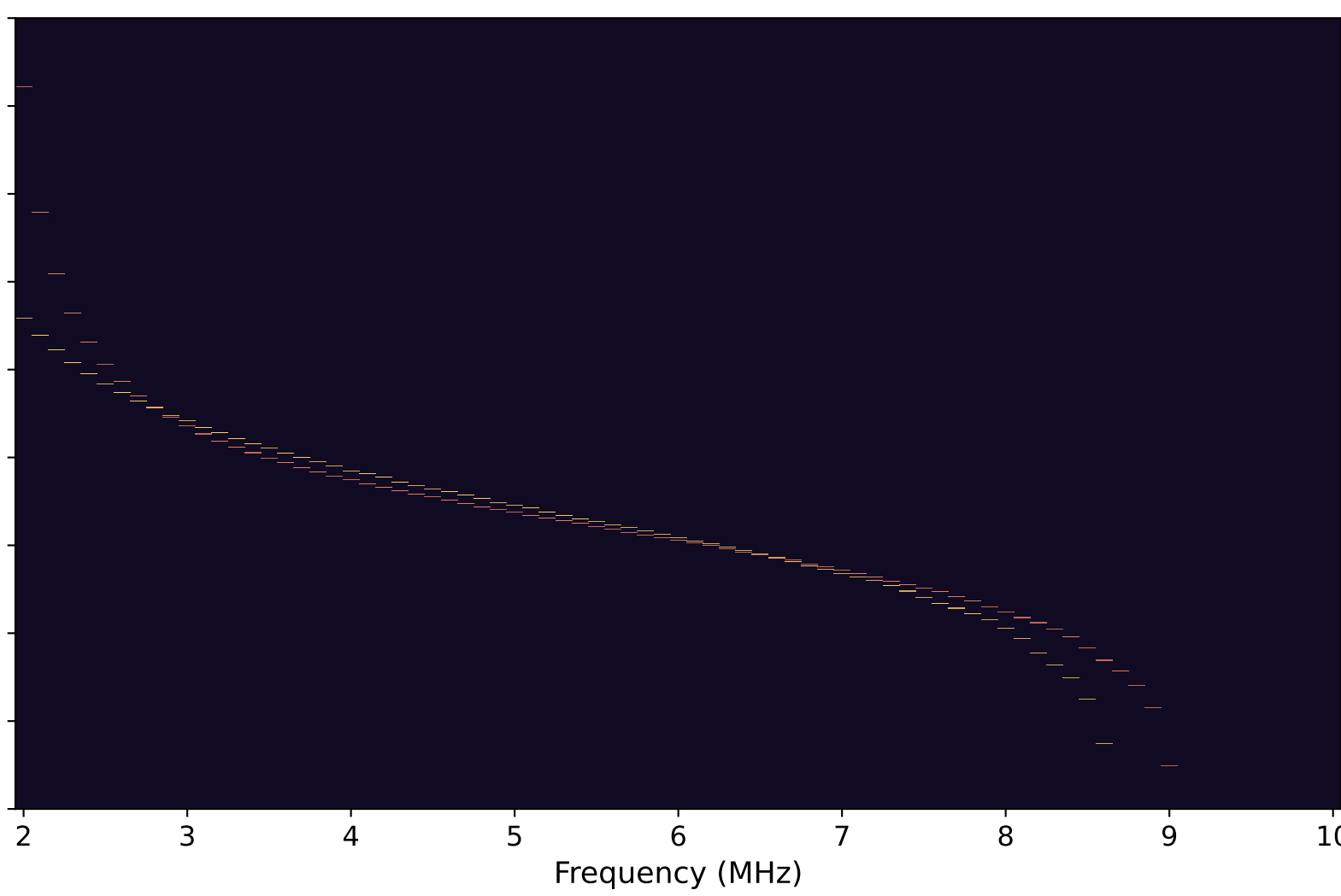
D Guarded half outer fan, 4 extra seeds · 211 returns · 71.7 s 105 anchor / 162 full directions · 211/211 reference returns matched
