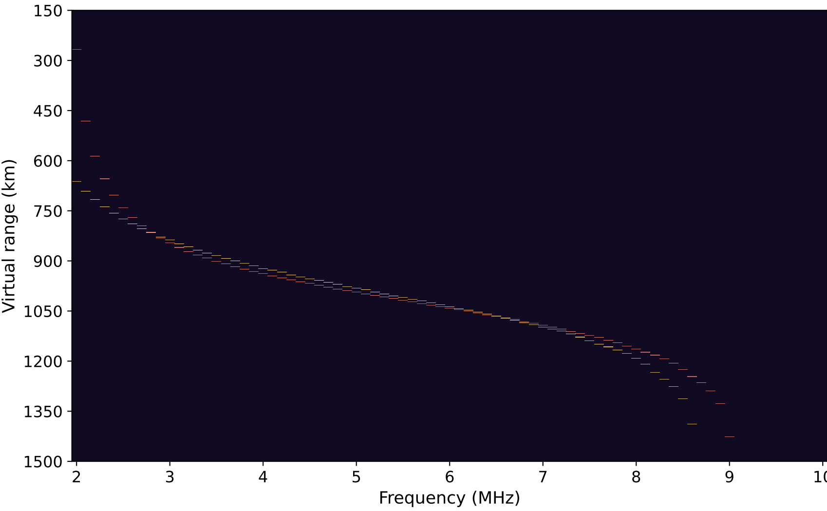
C Guarded half outer fan, 0 extra seeds · 211 returns · 40.7 s 105 anchor / 162 full directions · 211/211 reference returns matched
