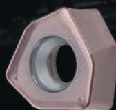
Indexable inserts for high feed rate milling cutters
