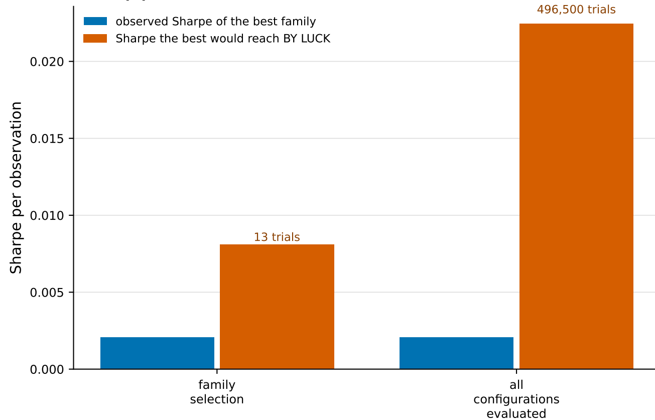
(a) The best result does not clear the luck benchmark
