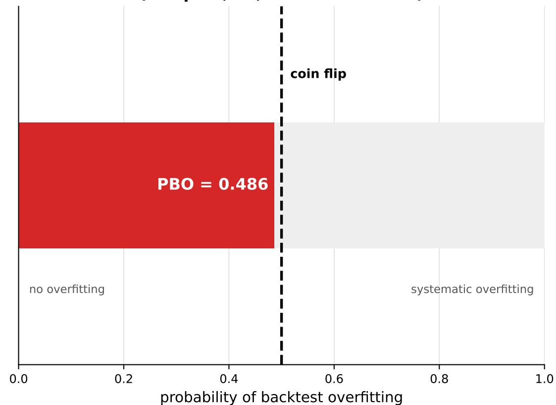
(b) Selection is uninformative (70 splits, 32,385 observations)
