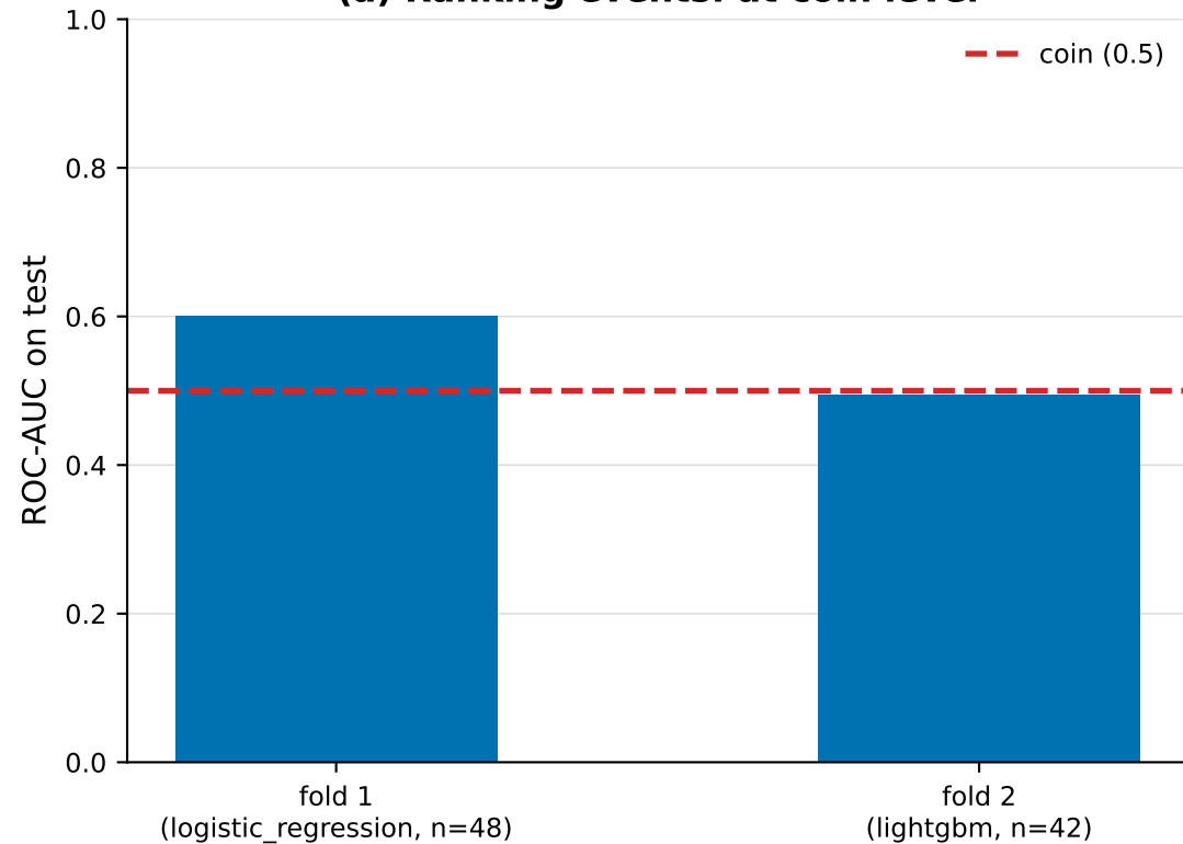
(a) Ranking events: at coin level
