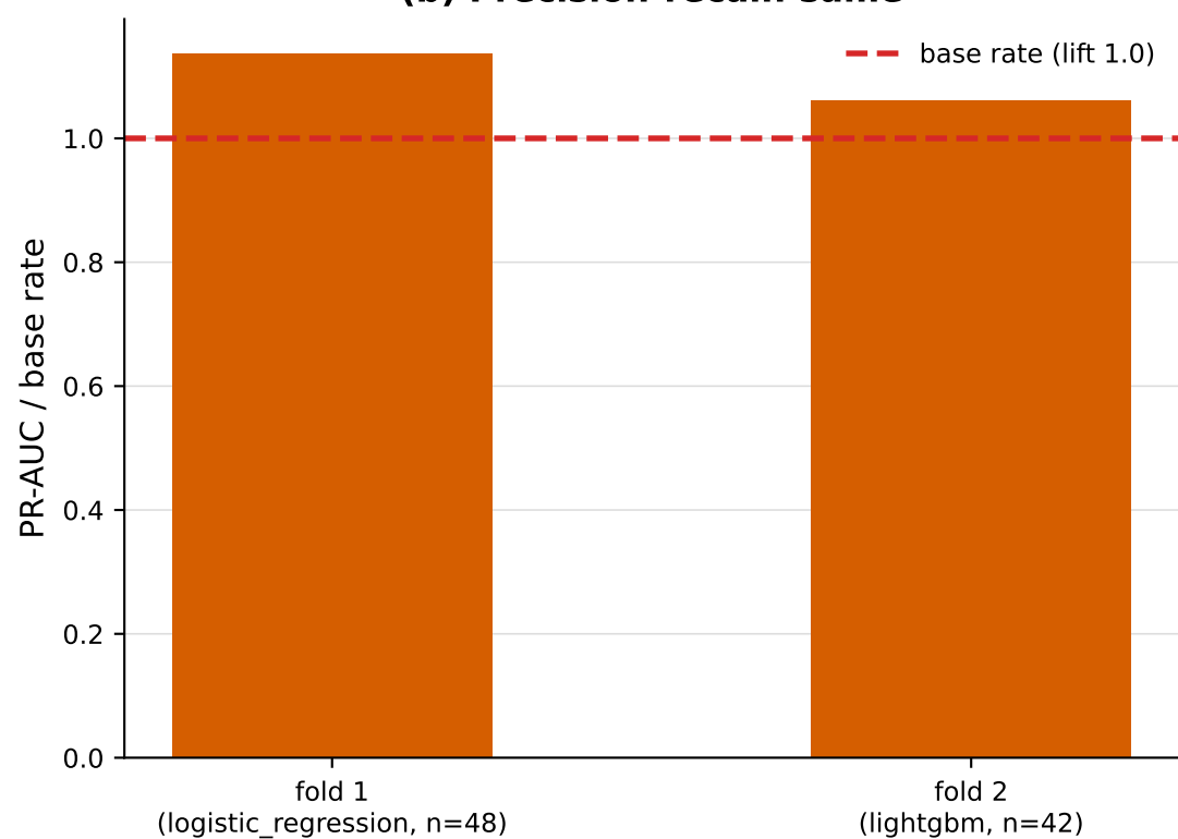
(b) Precision-recall: same
