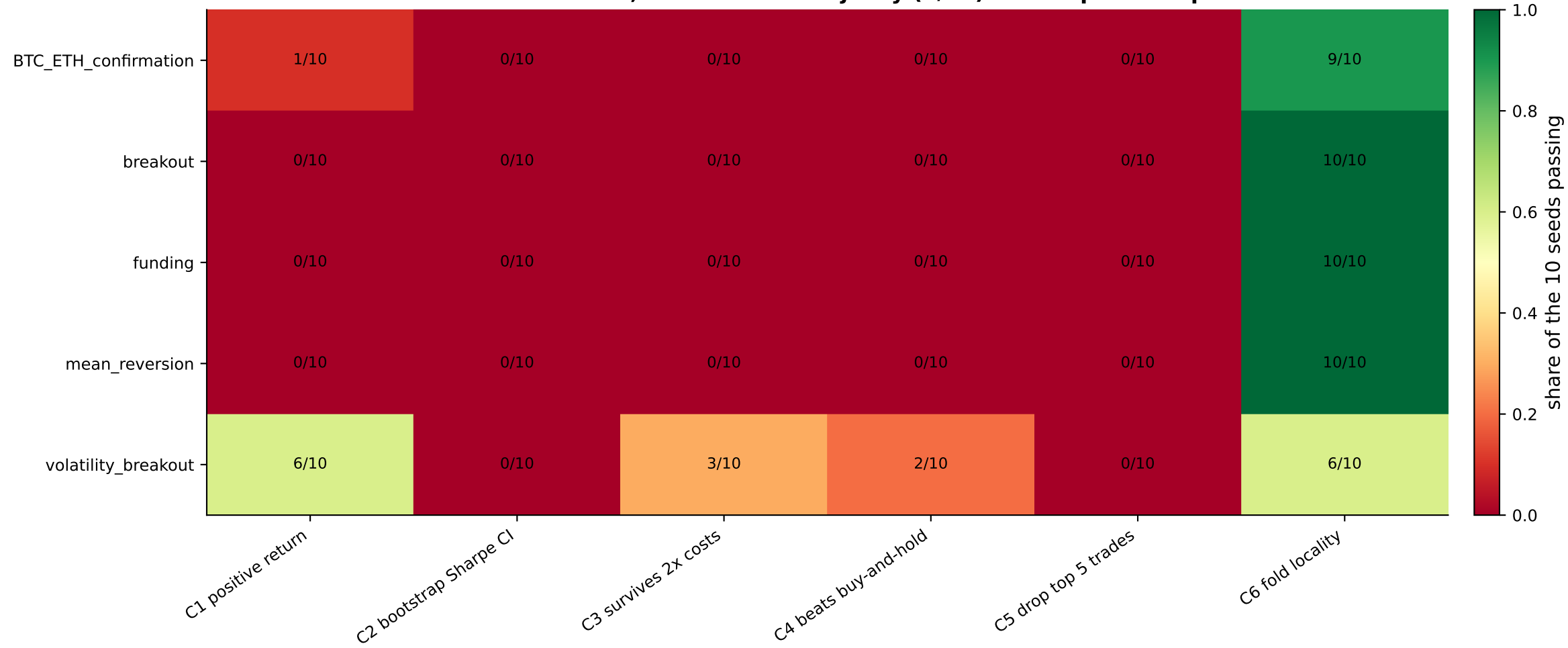
Promotion criteria, BTCUSDT - a majority (6/10) was required to pass
