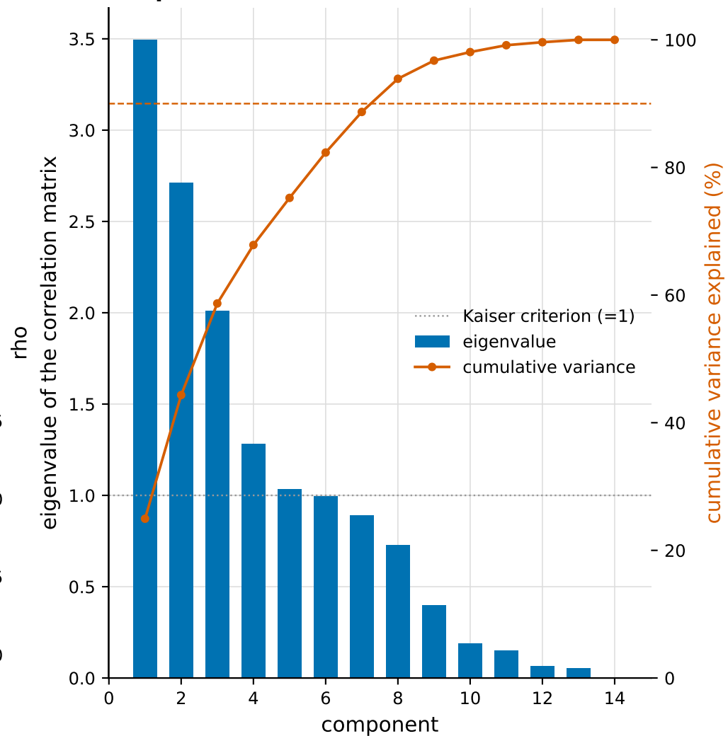
(b) Spectrum: 14 columns, effective rank 6.8
