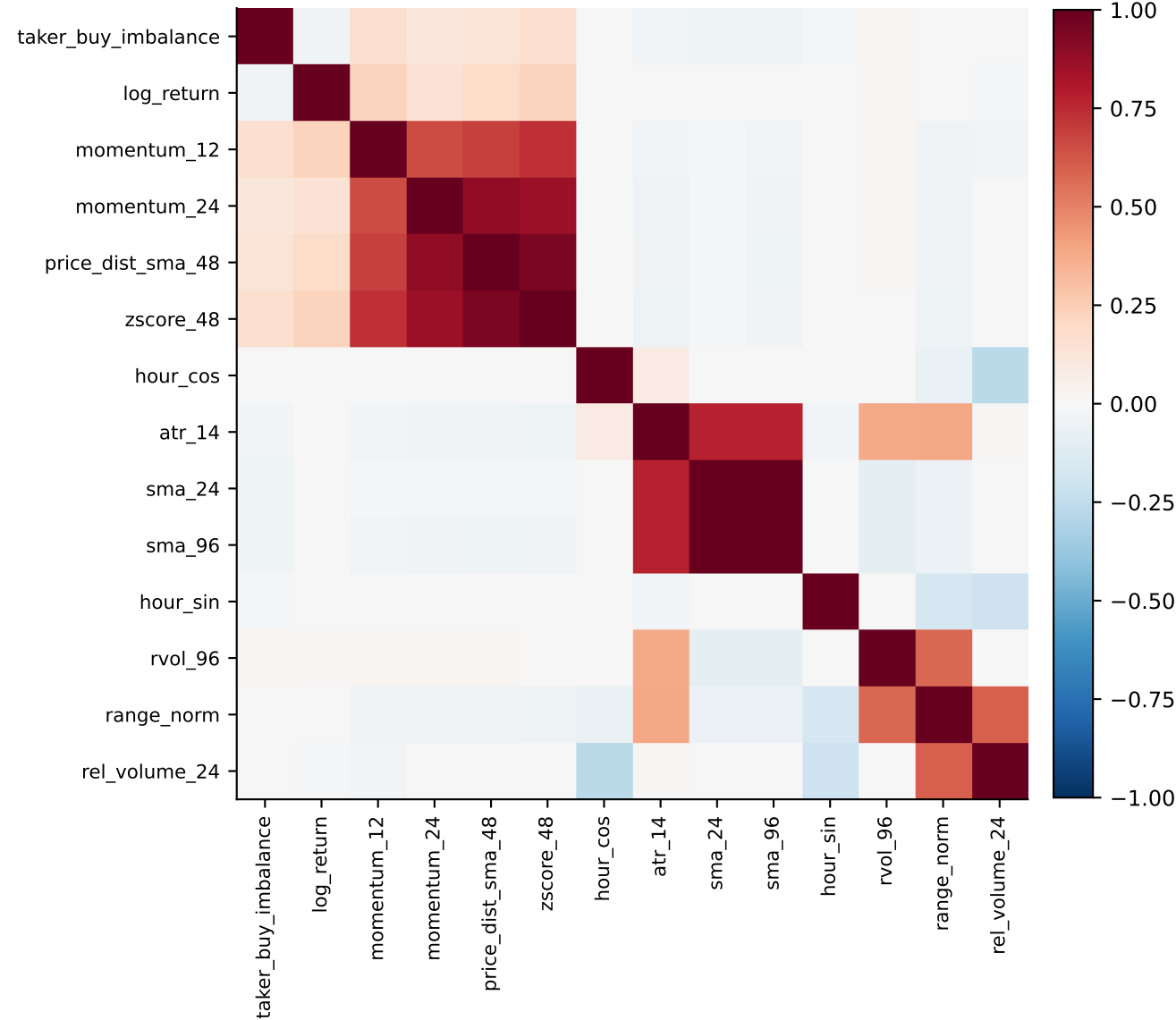
(a) Spearman correlation, hierarchically ordered
