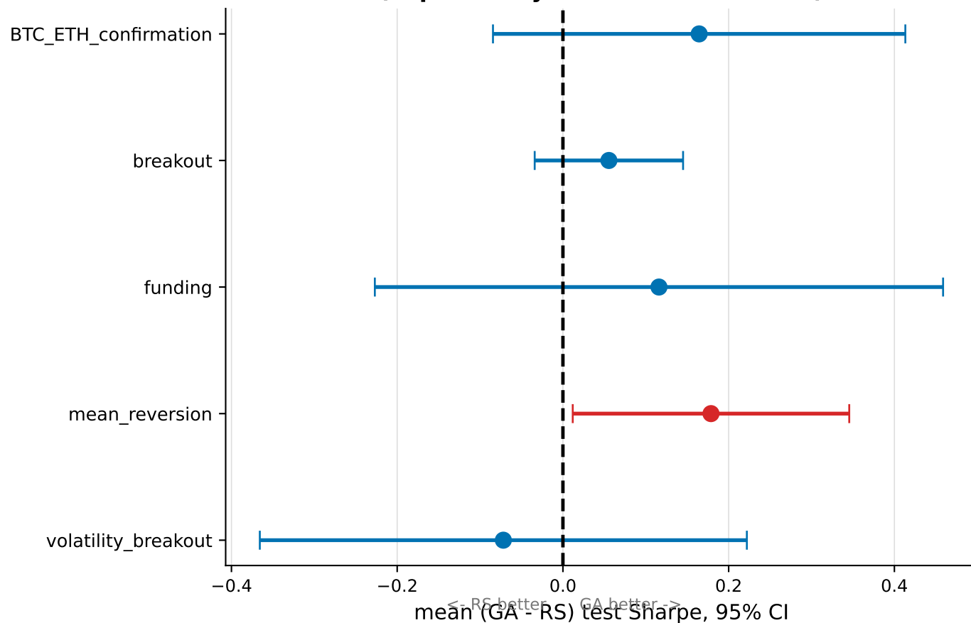
(b) 1 of 5 intervals exclude zero (expected by chance at 95%: 0.25)
