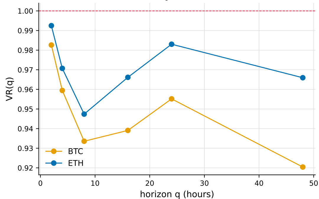
Lo-MacKinlay variance ratios
