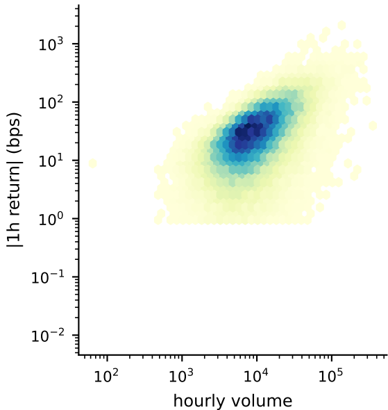
BTC · Spearman \rho = 0.528
