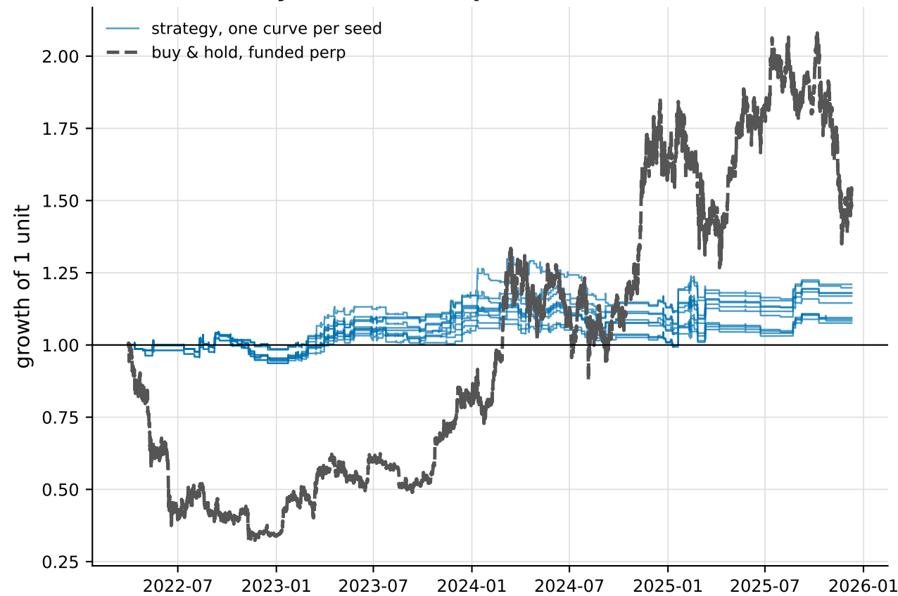
(a) pdl_reclaim_long BTC: 10/10 seeds end positive, yet no bootstrap CI excludes zero
