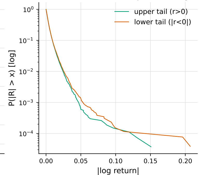
ETHUSDT - survival (complementary CDF)
