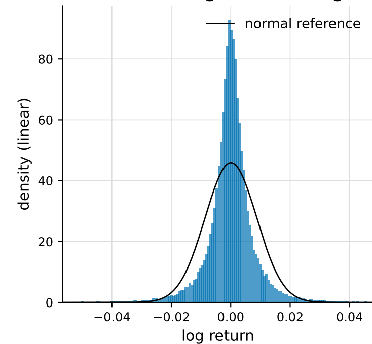
ETHUSDT - 1h log-return histogram
