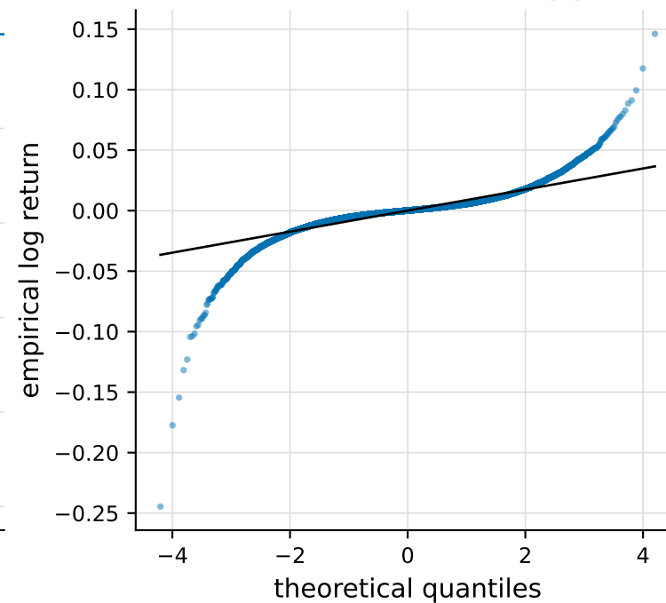
ETHUSDT - normal QQ
