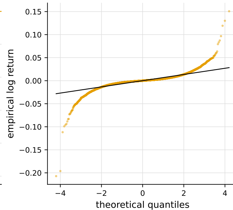
ETHUSDT - normal QQ
