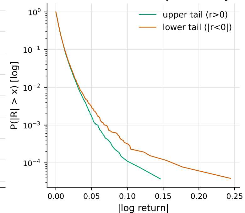
ETHUSDT - survival (complementary CDF)
