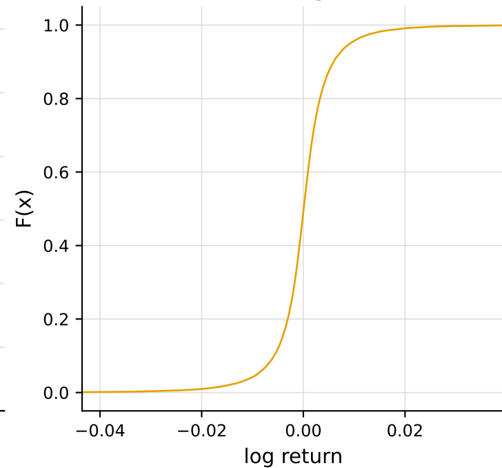
ETHUSDT - empirical CDF
