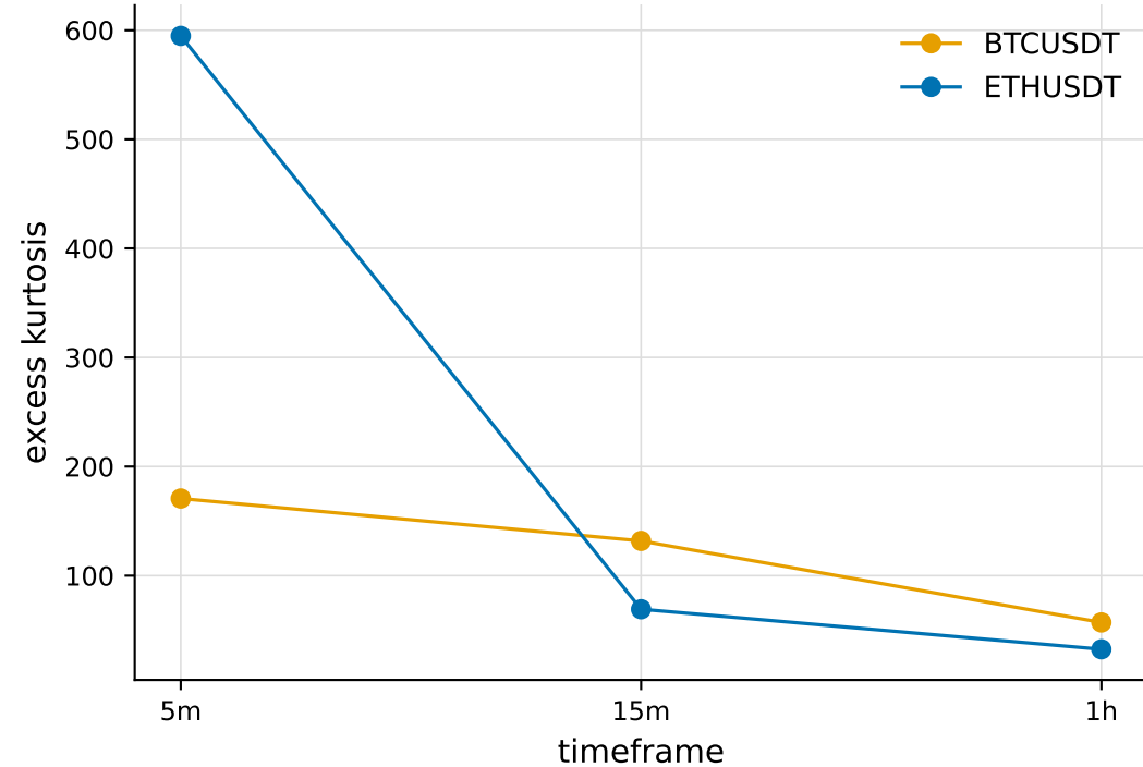
Excess kurtosis vs timeframe
