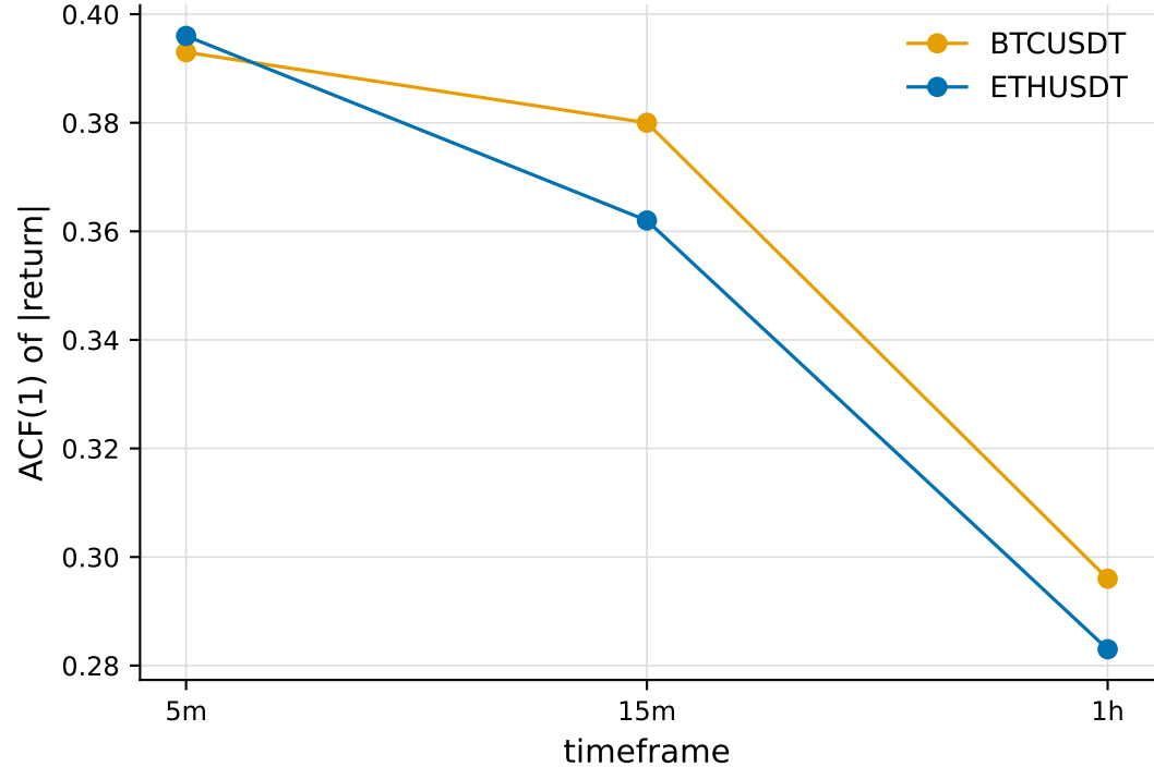
|return| lag-1 ACF vs timeframe
