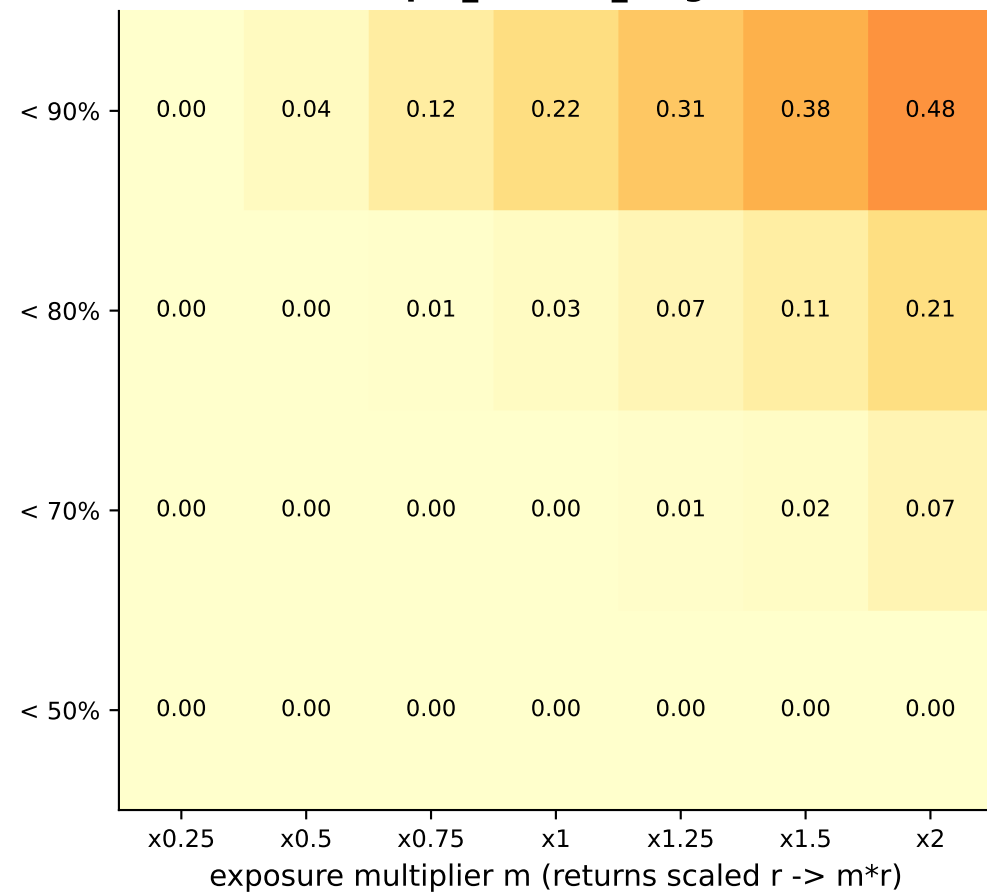
pdl_reclaim_long
