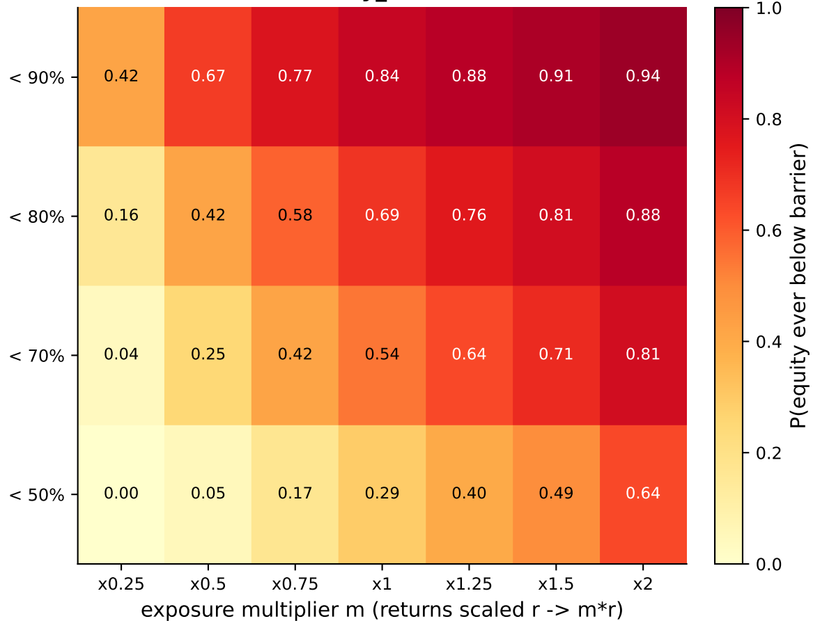
volatility_breakout
