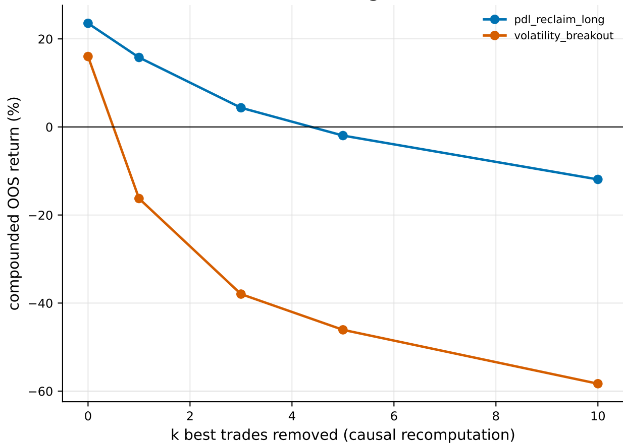
(b) Return after removing the k best trades
