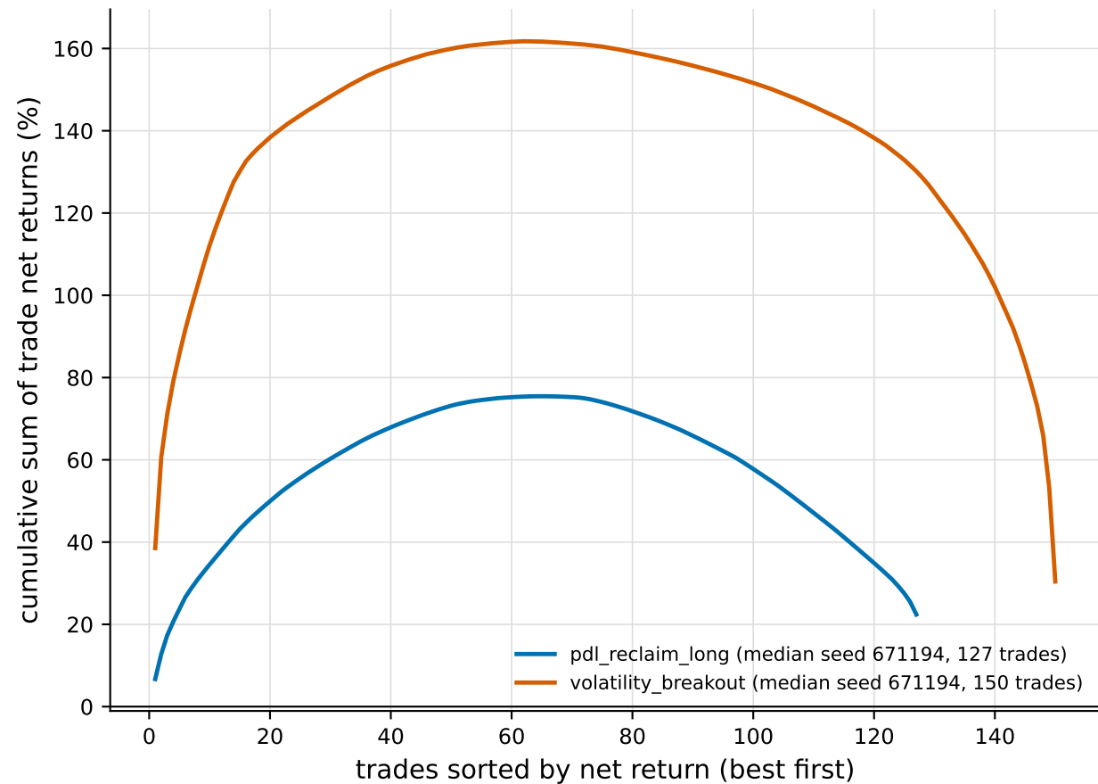
(a) Cumulative contribution of sorted trades
