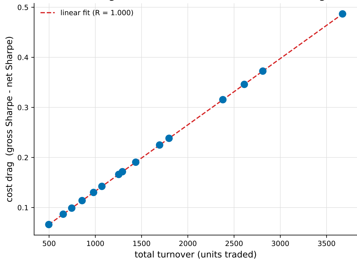
(b) The drag is a function of turnover, not of the signal
