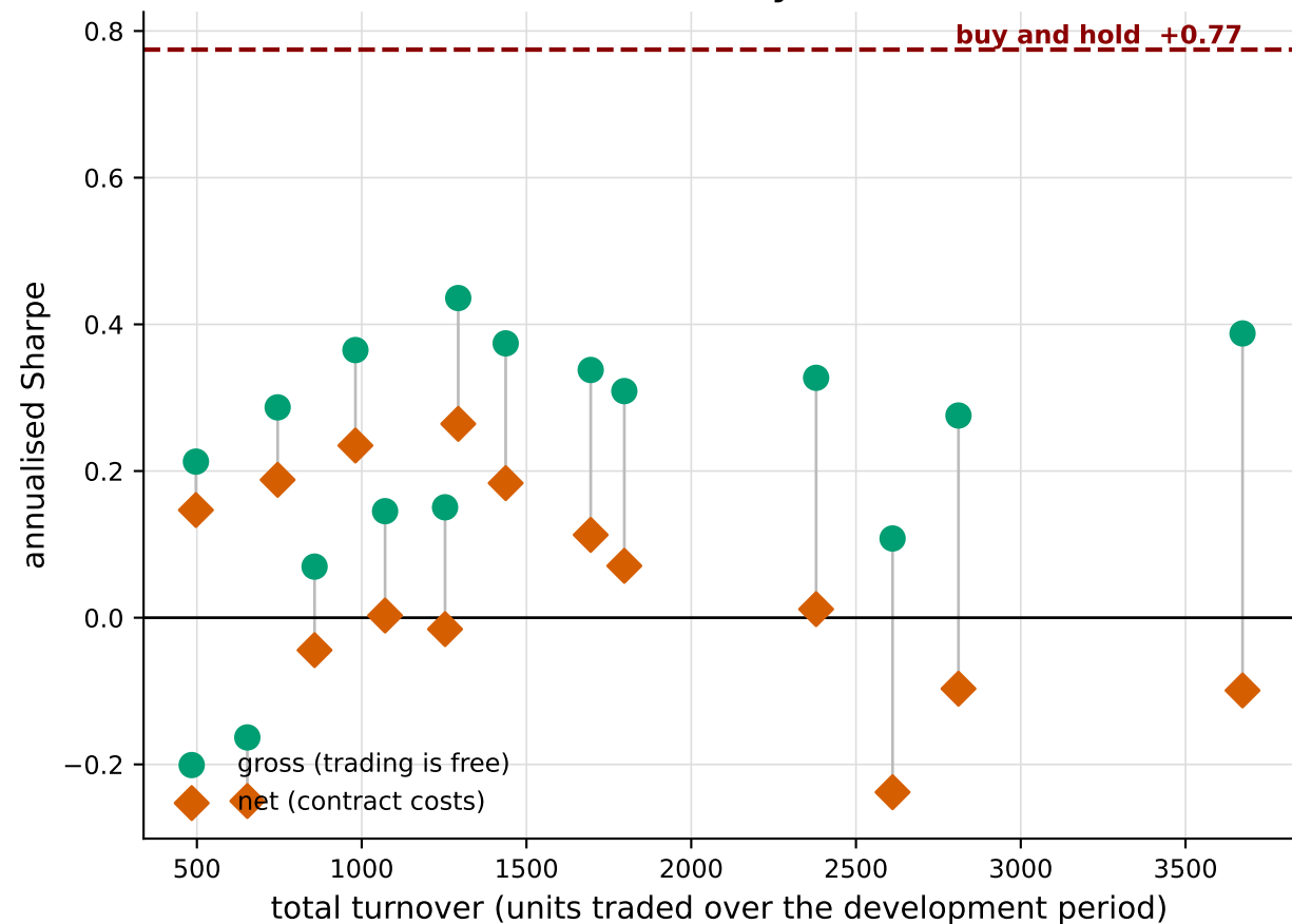
(a) Costs pull every parameterisation down; none reaches the buy-and-hold line
