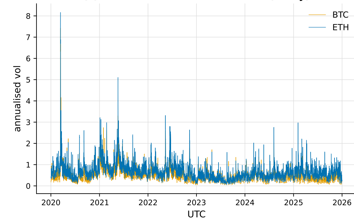
(c) Annualised vol co-movement (1-day)
