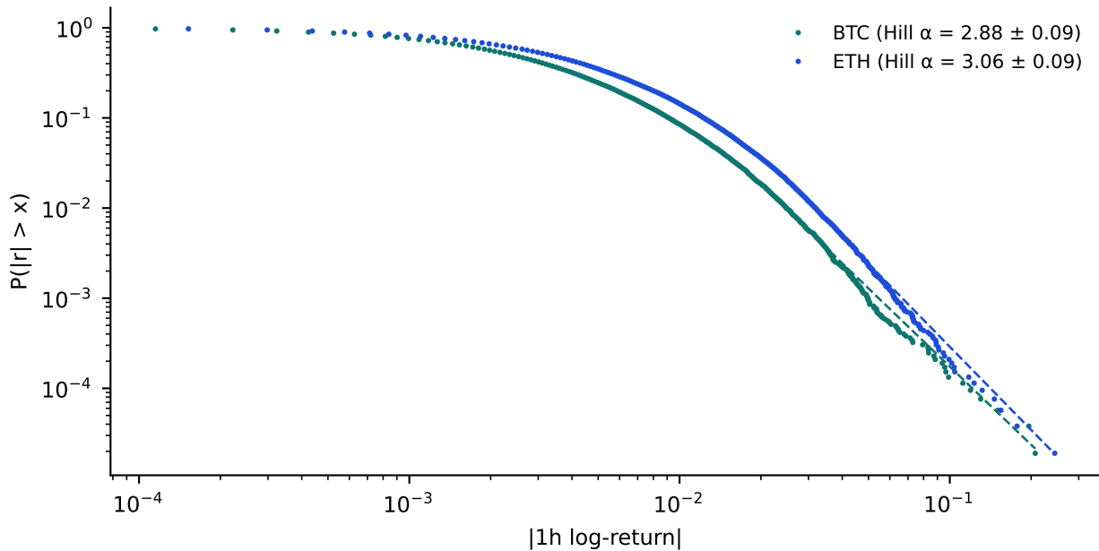
Empirical survival of absolute returns, log-log · dashed = Hill power-law fit
