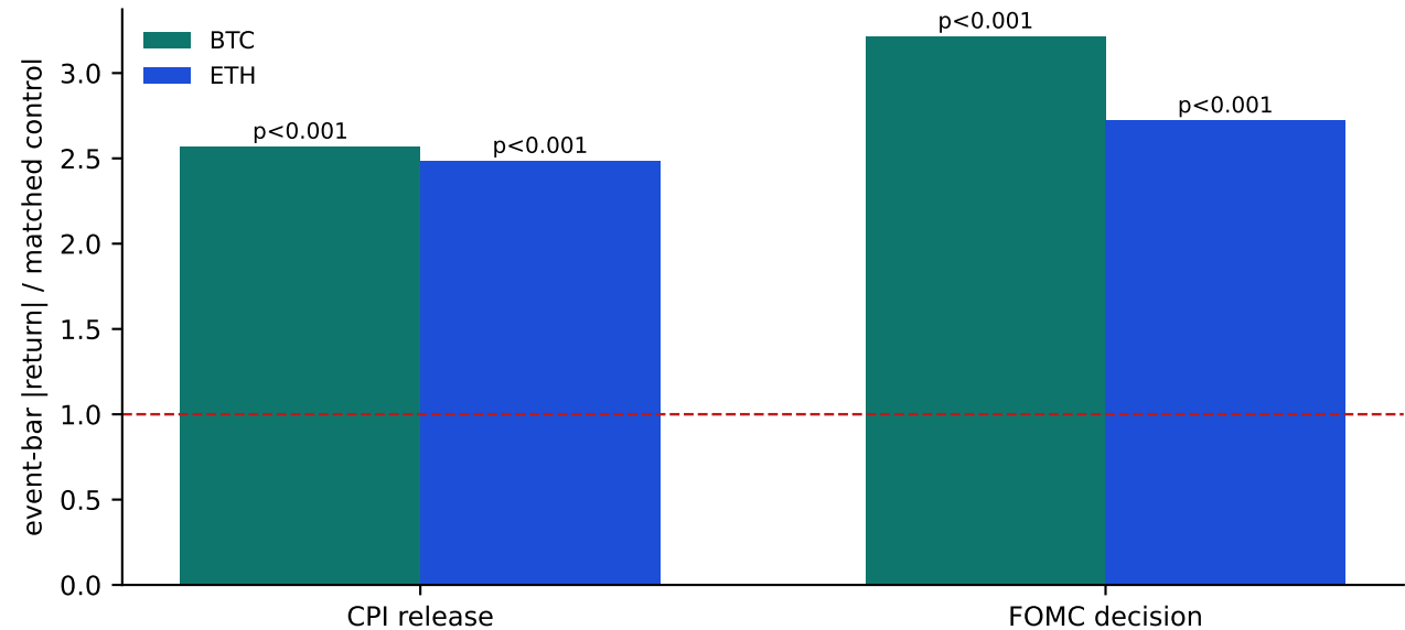
Event-hour volatility vs same-UTC-hour non-event bars · permutation p-values
