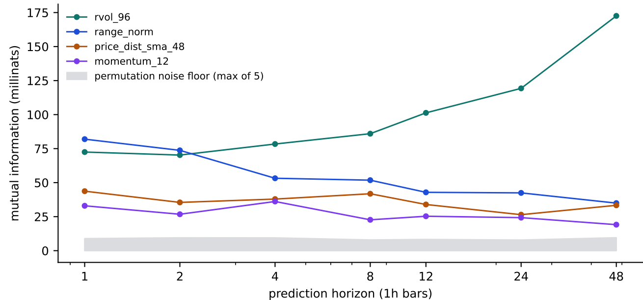
MI between strongest features and forward returns · BTC 1h, development
