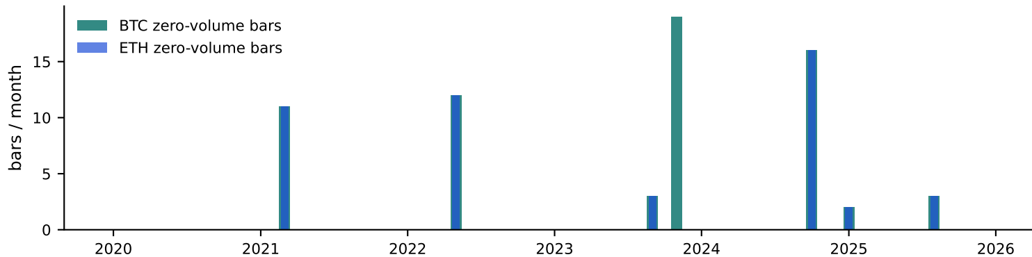
QC incidents: zero-volume 5m bars — flagged, kept, never repaired
