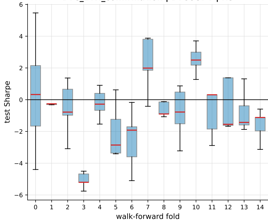
(b) Ten seeds, one fold: the spread within each box BTC_ETH_confirmation | BTCUSDT | RS
