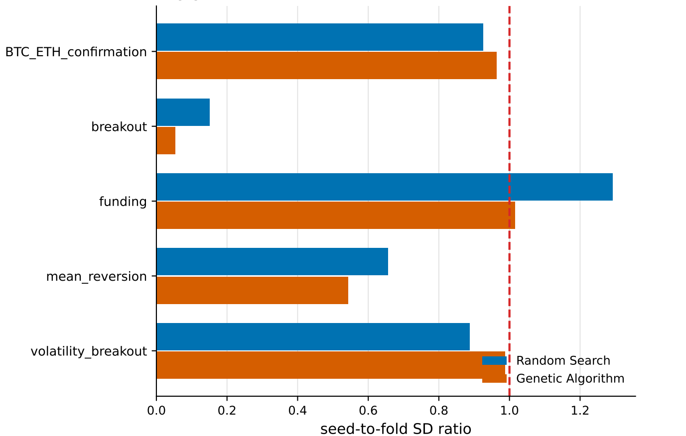
(a) How much of the answer is the random seed?
