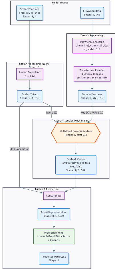
Figure 1: Model Architecture with Cross-Attention
