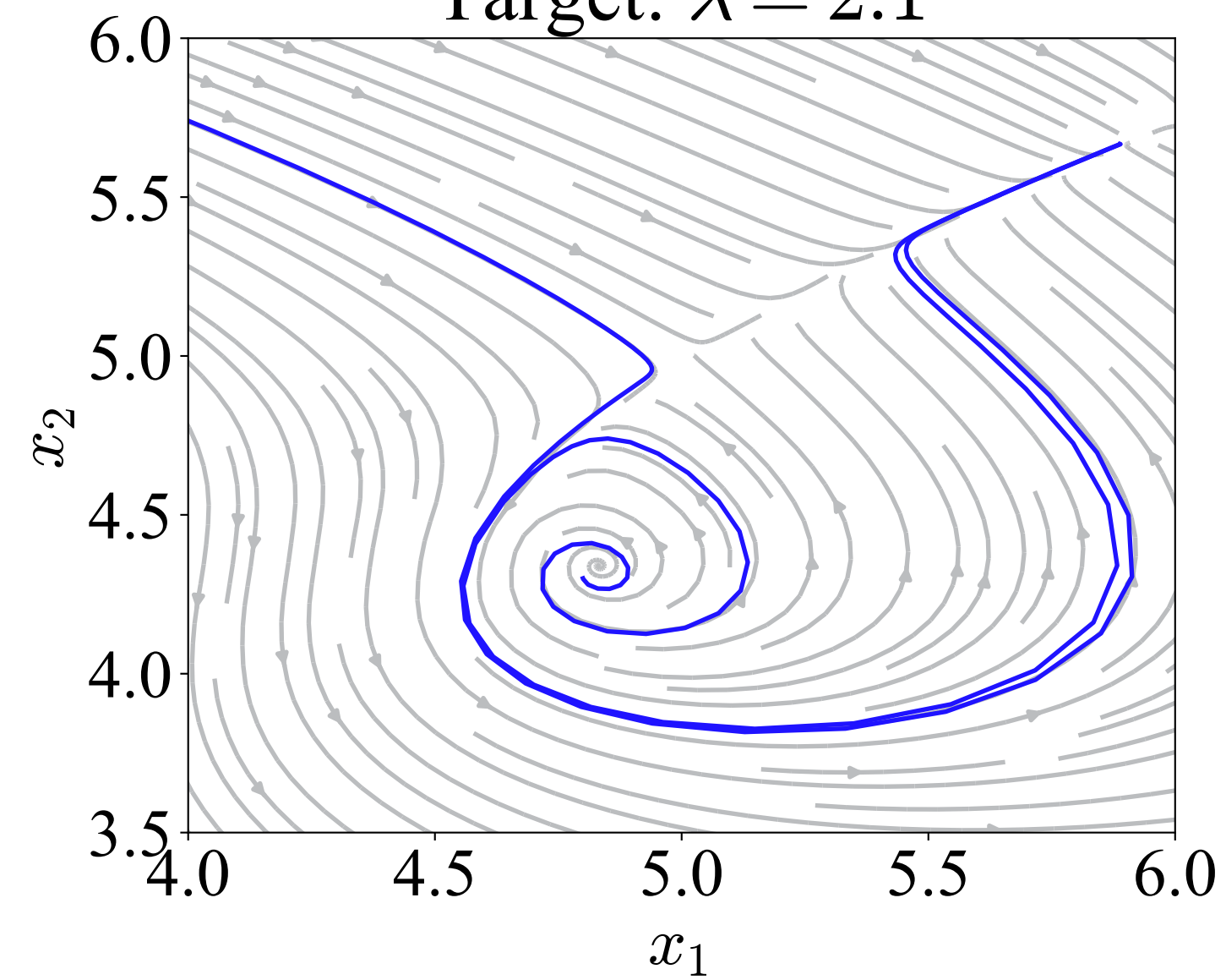
RNCRN: \lambda = 2.1
