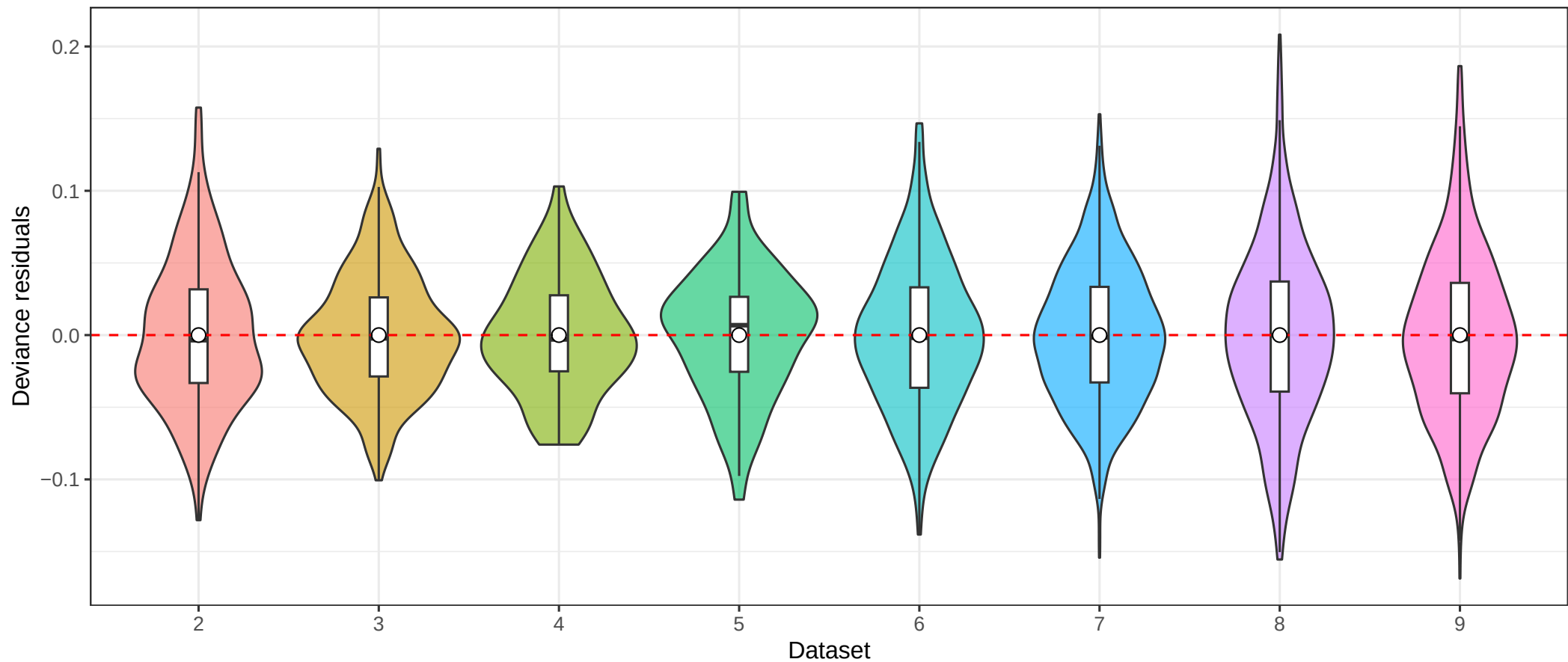
Model residuals by dataset (centred on 0 = no site bias)
