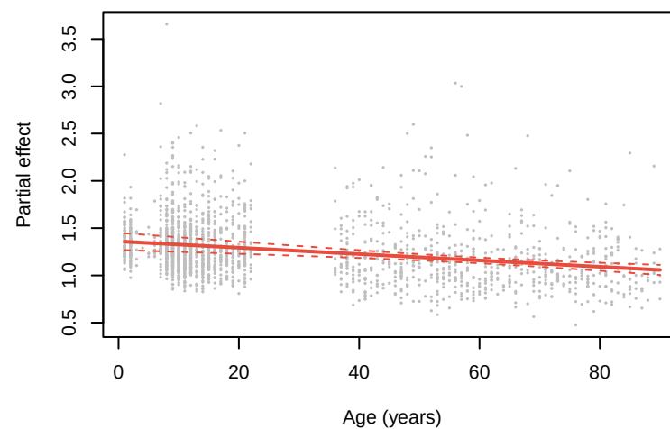
R24 | edf=6.4 | q=0.000
