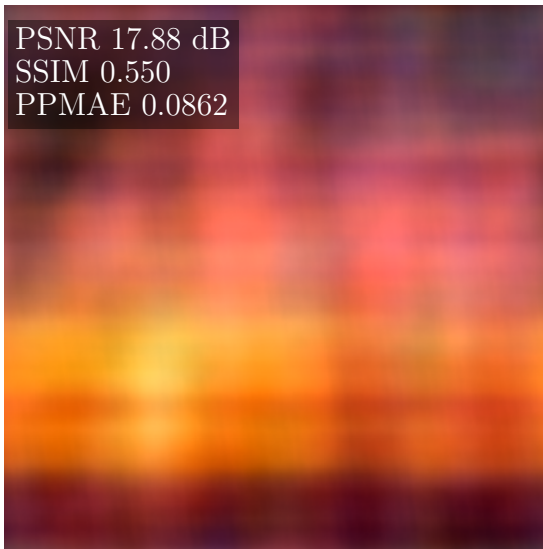
Zero-Filled
