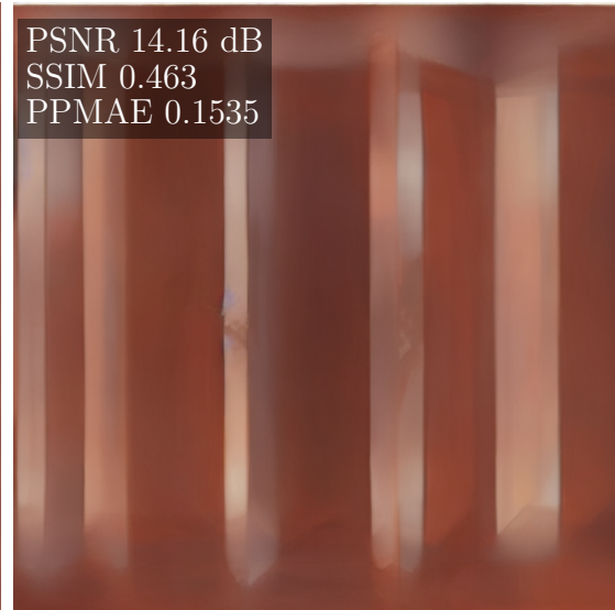
c_r = ""
