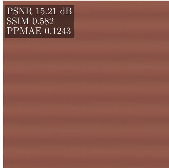
Zero-Filled
