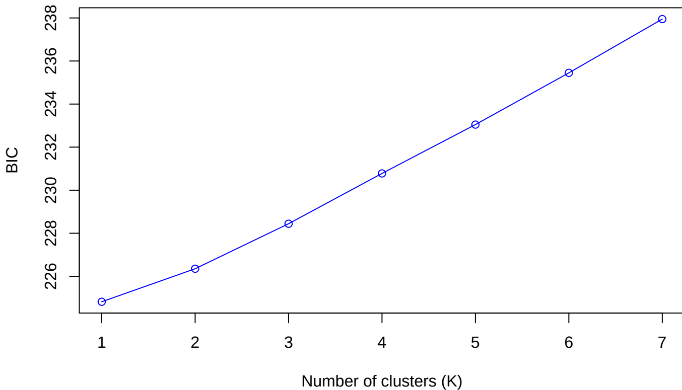
Value of BIC versus number of clusters WBNP: 1986 – 1999
